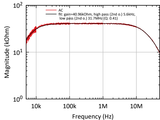
Fig. 4: AC output: AC transfer function with silicon photodiodes, measured with 50 \Omega load.
