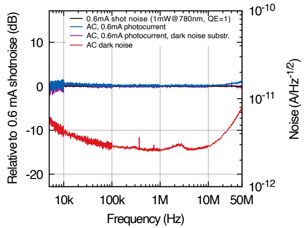
Fig. 2: AC output: Dark noise and bright noise calibrated to photocurrent with the transfer function below, measured with 50 \Omega load.
