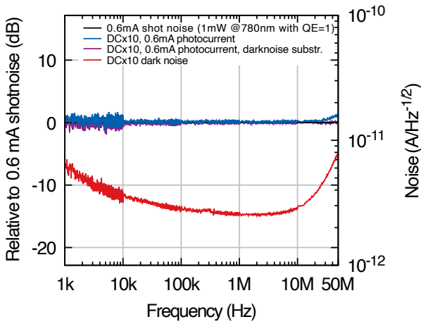
Fig. 1: DC x 10 output: Dark noise and bright noise calibrated to photocurrent with the transfer function below, measured with 1 M \Omega load.
