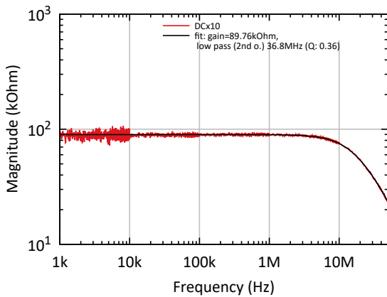
Fig. 3: DC x 10 output: DC x 10 transfer function with silicon photodiodes, measured with 1M \Omega load.
